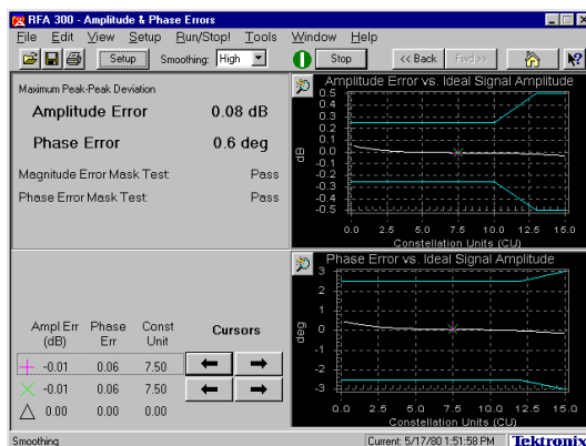
In-band flatness < ±0.08 dB Phase Error < 0.7 degrees
